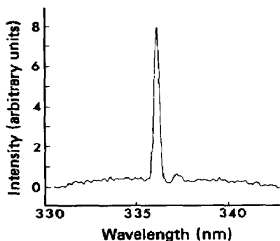
Fig. 1. Spectrum observed during irradiation of partially dissociated H_2 using an ArF laser: resolution, about 0.4 nm (full width at half-maximum); cell pressure, 1 Torr.
