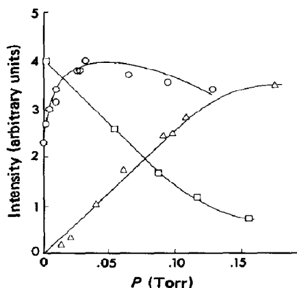
Fig. 2. Variation in the \text{NH} emission intensity with reactant partial pressure: \circ , [\text{NO}] ; \triangle , [\text{H}] calculated by assuming 90% dissociation of \text{H}_2 in a large excess of argon carrier; \square , 0.1 [\text{H}_2] .
